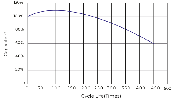
Cycle Life vs Remaining Capacity@25°C(77°F)
